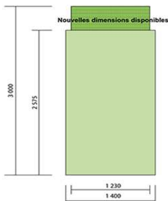
Bloc-porte 1 vantail
